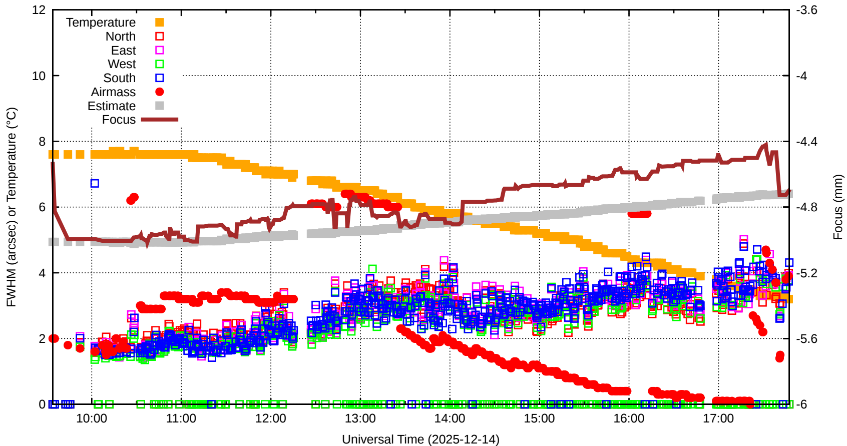
FFT (FWHM-FOCUS-TEMP) Monitoring
